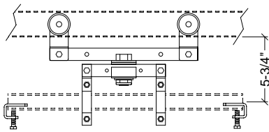
10 PIVOT DEVICE
