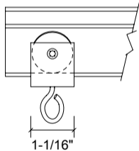
701 SINGLE CARRIER
