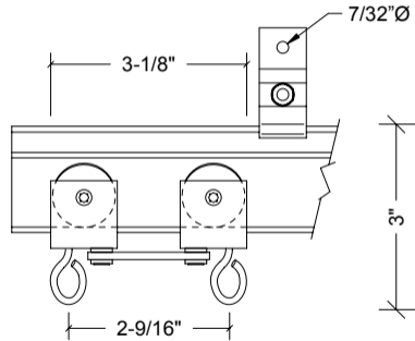
702 MASTER CARRIER
