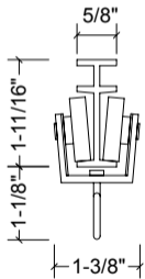
701 SINGLE CARRIER
